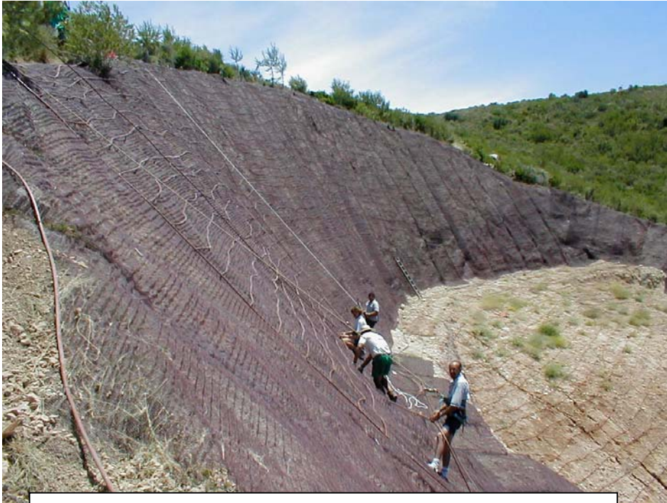
3. Fixing the mesh and the watering lines
